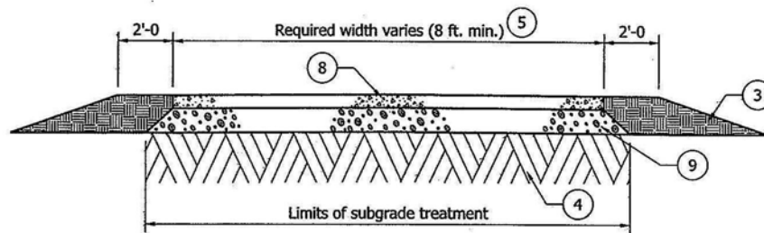
PCCP TYPICAL SECTION
